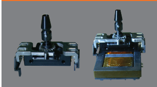
• Gripper nozzle
